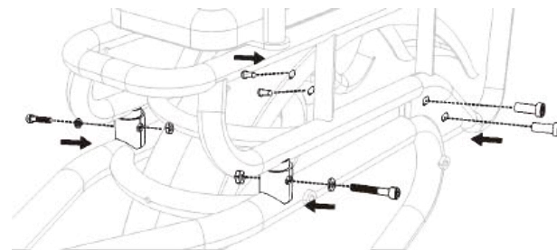
Place the rear rack onto the frame, then tighten the screws.
