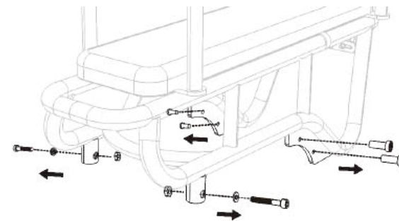
Remove the screws from the rear rack
